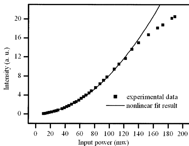
Figure 6. The output fluorescence intensity vs. the input power for 2 in THF with c = 1.0 \cdot 10^{-3} M
