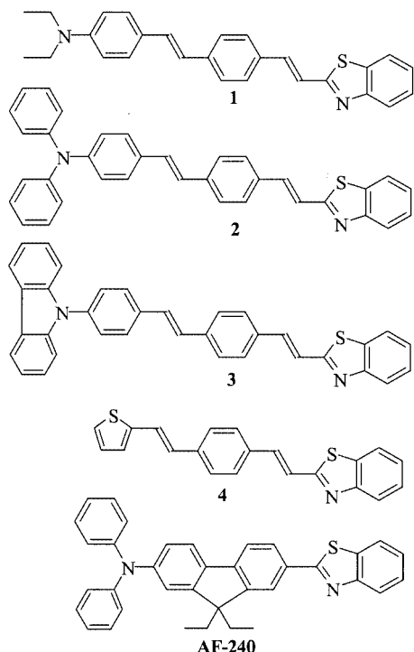
Scheme 1. Molecular structures of the compounds studied in this work and of AF-240 [10]
