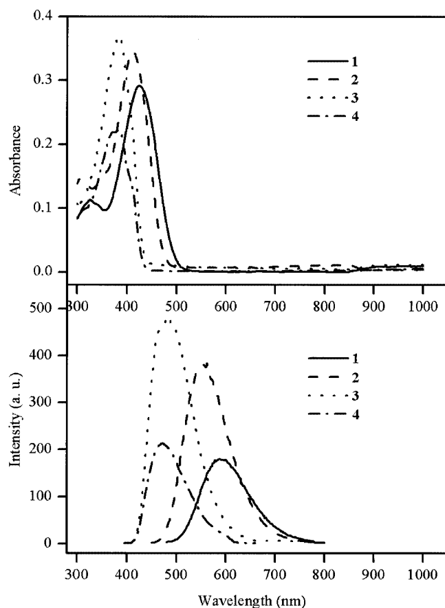
Figure 3. Linear absorption and single-photon-excited fluorescence in THF at c = 5.0 \cdot 10^{-6} M
