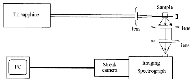
Figure 5. Experimental setup for TPEF measurement
