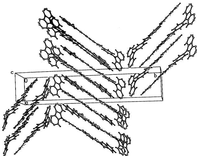
Figure 2. Packing diagram for 3 viewed along the c axis
