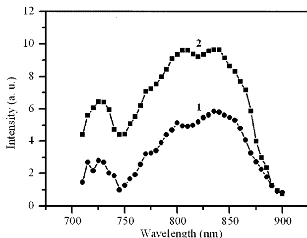
Figure 7. Two-photon excitation (TPE) spectra of 1 and 2 in THF with c = 1.0 \cdot 10^{-3} M
