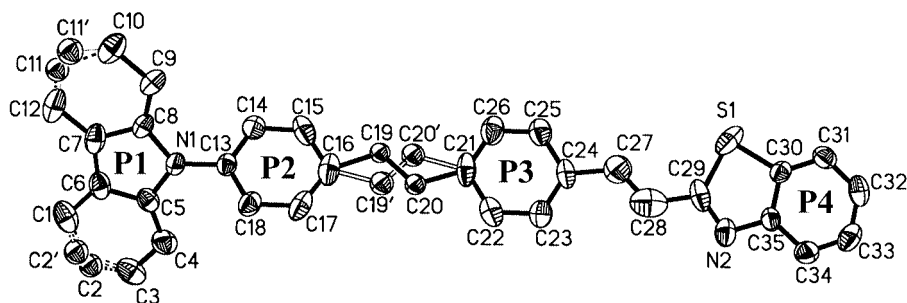
Figure 1. Molecular structure of 3 . Hydrogen atoms have been omitted for clarity
