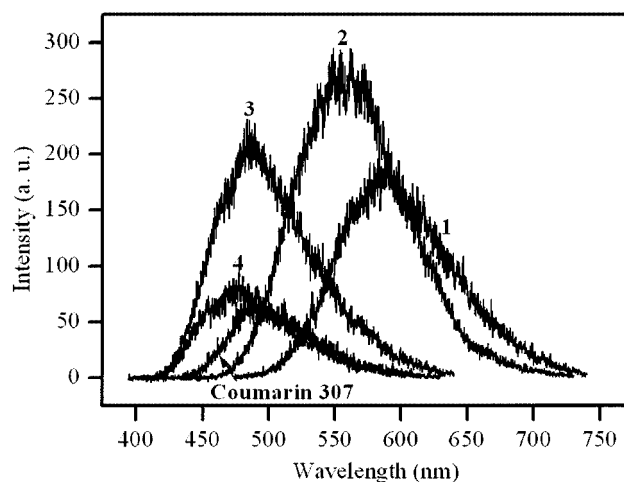
Figure 8. Two-photon-excited fluorescence spectra of the compounds in THF and of Coumarin 307 in MeOH at c = 1.0 \cdot 10^{-4} M
