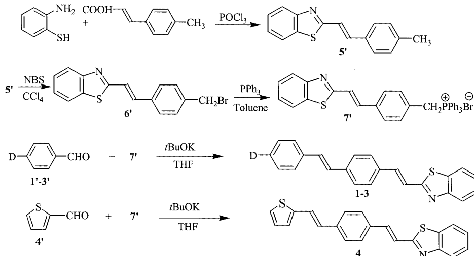
Scheme 2. Synthetic strategy for the preparation of the compounds (D = diethylamino, diphenylamino, carbazoyl)
