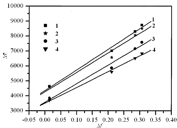
Figure 4. Stokes shift \Delta\tilde{\nu} vs. orientation polarizability \Delta f of the solvents. (The scatter dots are the experimental data and the lines are the linearly fitted results.)
