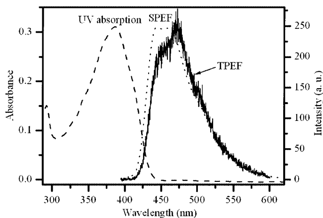
Figure 9. The UV absorption and single-photon-excited fluorescence (SPEF) spectra ( c = 5.0 \cdot 10^{-6} M) and the two-photon-excited fluorescence (TPEF) spectrum ( c = 1.0 \cdot 10^{-4} M) of 3 in toluene
